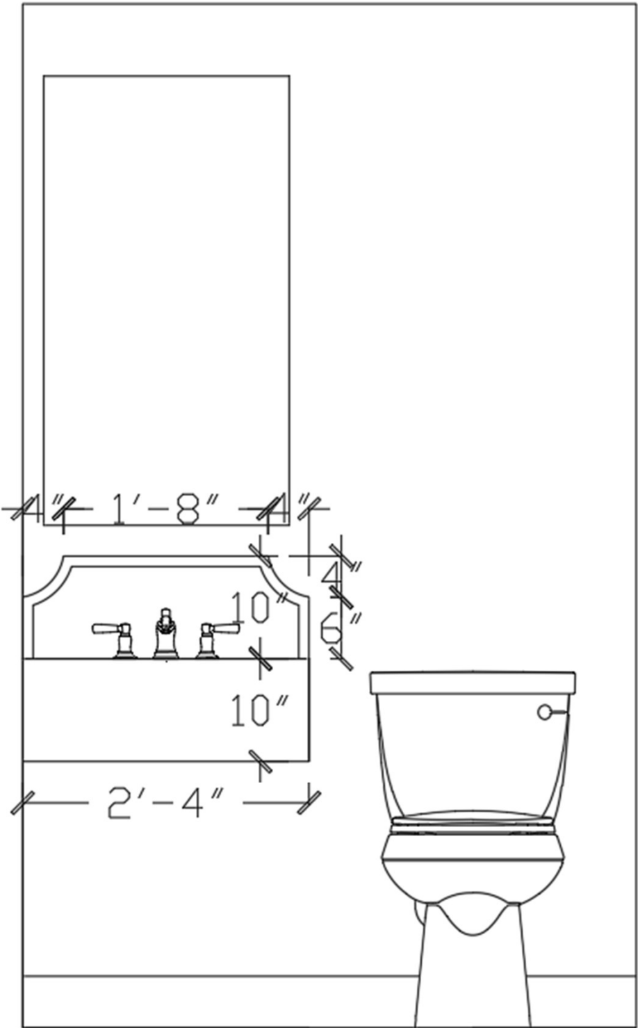
VANITY ELEVATION WITH DIMENSIONS
